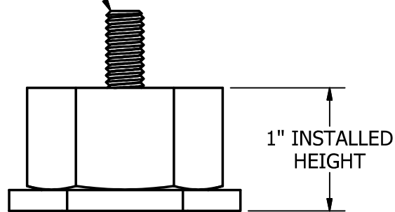
Dimensioned Metal Roof Base Assembly
