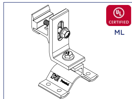
S-5! VersaBracket with Ultra Rail hardware
