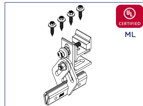
S-5! ProteaBracket with Ultra Rail hardware
