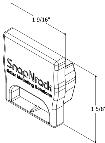
Dimensioned UR-40 Rail End Cap
